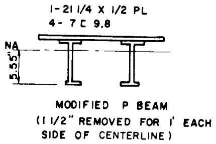
Fig. 1—Elevation and sections of beam strips.
